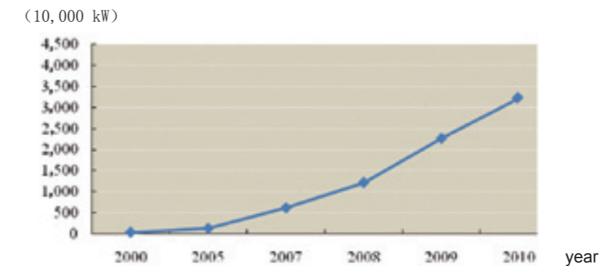
Figure 4-6 Installed wind power capacity in China
